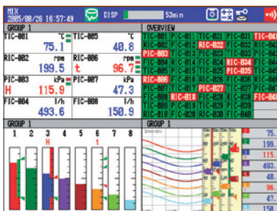
– Split screen display – This mode lets you split the screen into four areas, and select the display format for each of the areas.
