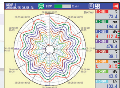
– Circular display – In addition to the normal T-Y trend display, circular display is possible (DX2000 only).
