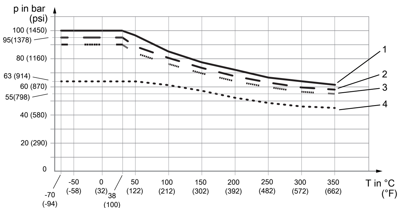
Fig. 10: Allowed process pressure as a function of process connection temperature
