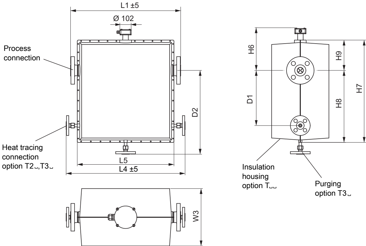
Fig. 21: Dimensions in mm: version with insulation housing for meter sizes Intense 34, 36 and 38 only
