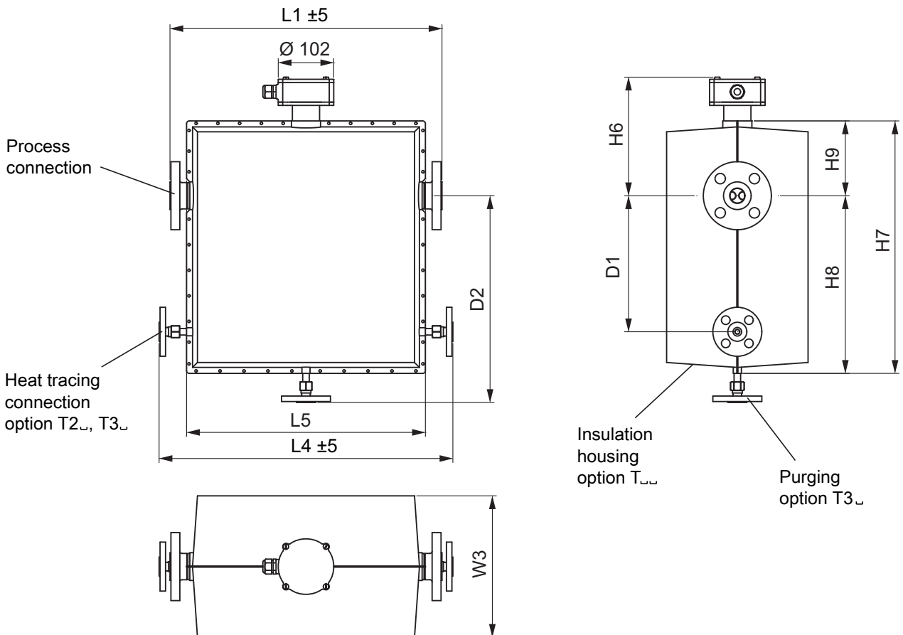
Fig. 26: Dimensions in mm: version with insulation housing for meter sizes Intense 34, 36 and 38 only
