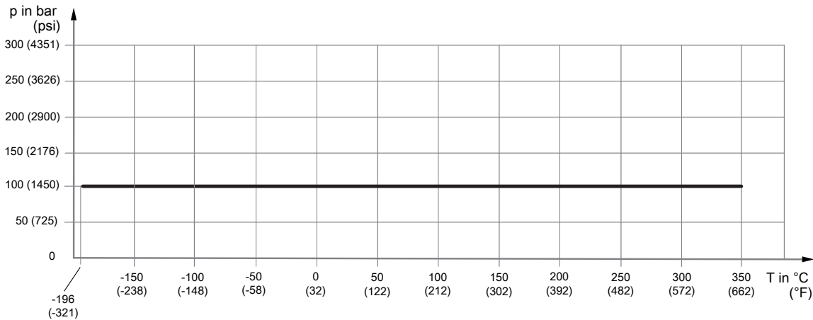
Fig. 16: Allowed process pressure as a function of process fluid temperature
