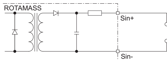
Fig. 44: Status input connection
