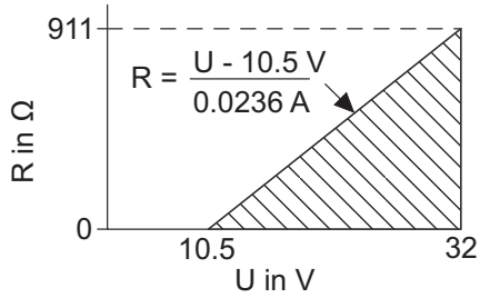
Fig. 30: Maximum load resistance as a function of an external power supply voltage
