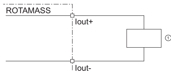
Fig. 29: Active current output connection lout HART
