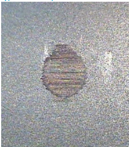
Figure 4 Typical wear dimple after 15 min
