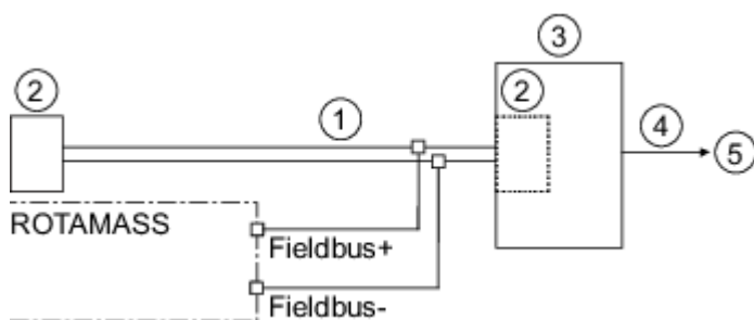
Fig. 35: PROFIBUS PA connection
