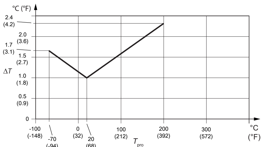
Fig. 5: Temperature accuracy
