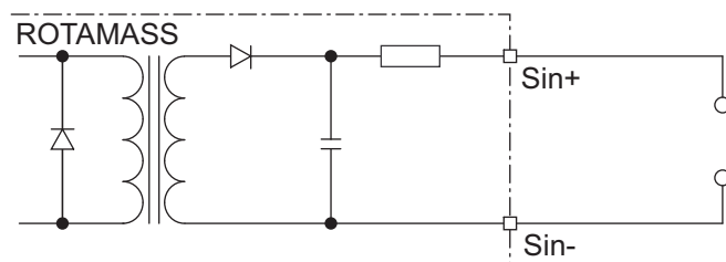
Fig. 34: Status input connection
