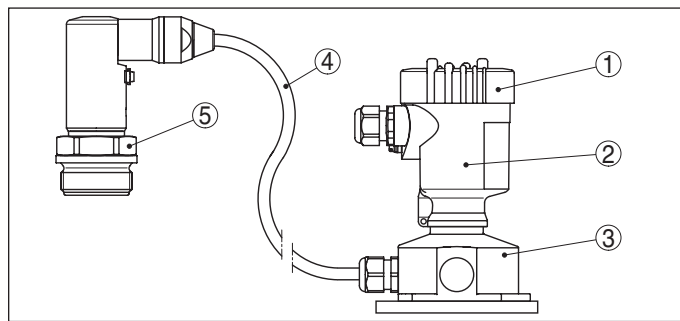
Fig. 11: Example of a VEGABAR 82 with protection rating IP 68 and external electronics
