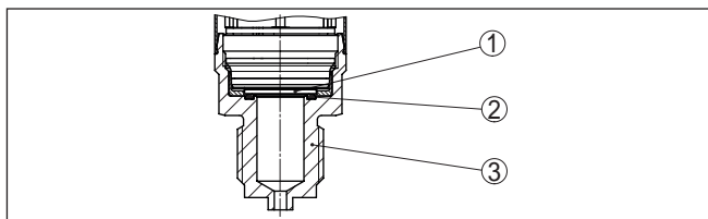
Fig. 5: Recessed installation of the measuring cell (example: thread G\frac{1}{2} , EN 837 manometer connection)
