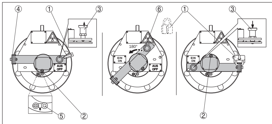
Fig. 31: Switching the radiation on - VEGASOURCE 31 version B
