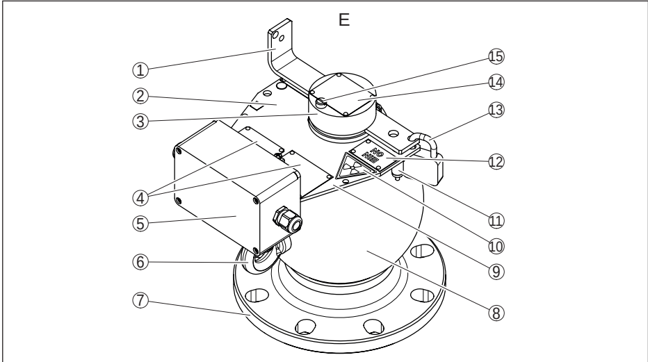
Fig. 42: Materials VEGASOURCE 31 - Version E
