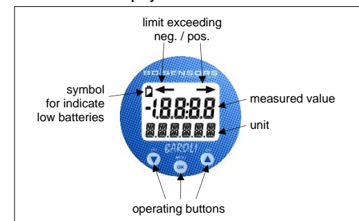
Fig. 4 Touch pad
