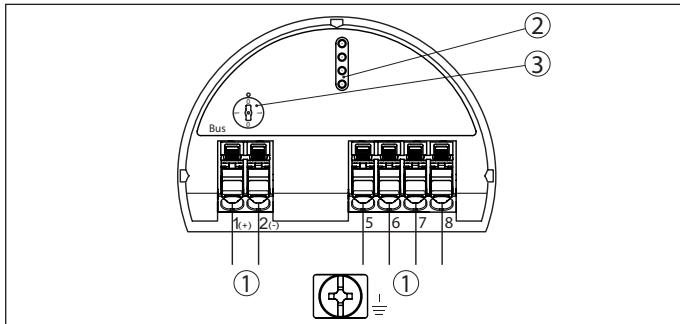
Fig. 18: Electronics and connection compartment - single chamber housing
