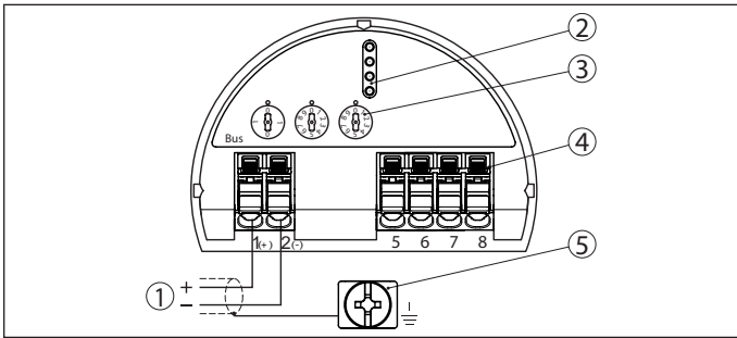
Fig. 15: Electronics and connection compartment - single chamber housing
