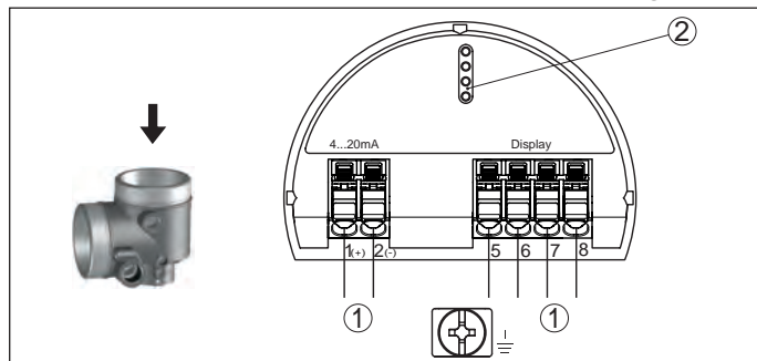
Fig. 12: Electronics compartment - double chamber housing
