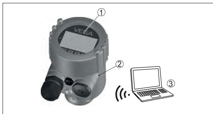
Fig. 25: Connection of the PC via Bluetooth USB adapter
