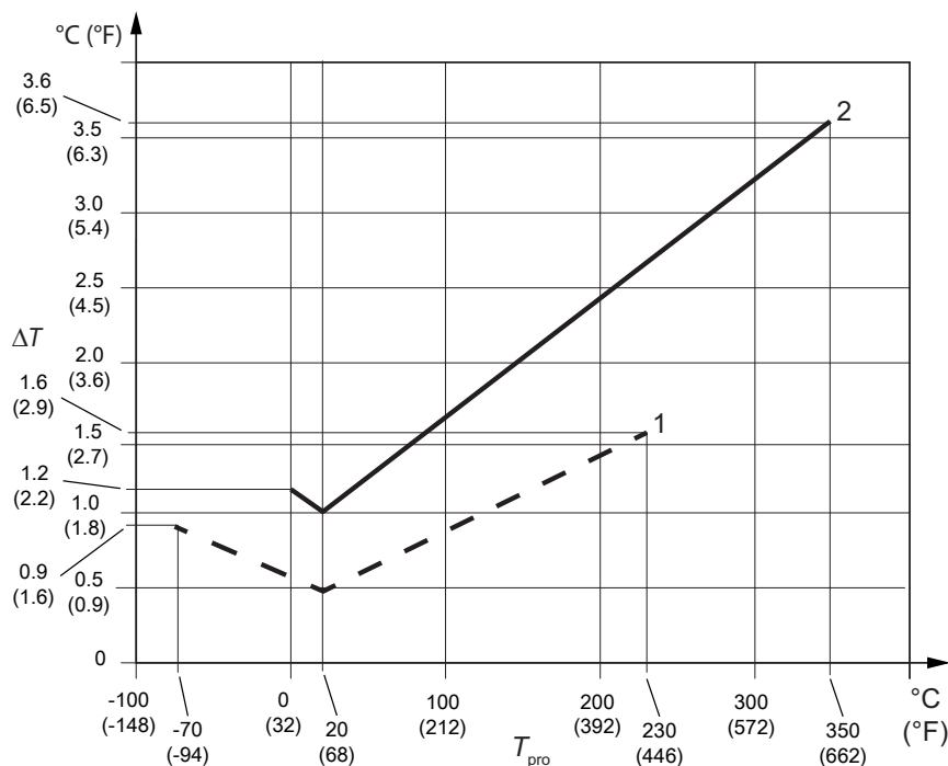
Fig. 6: Presentation of temperature accuracy
