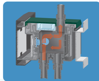
Flash window structure
